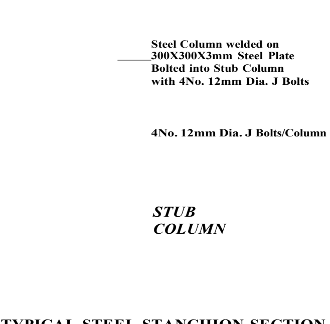
TYPICAL STEEL STANCHION SECTION (22No.) Scale 1:25
